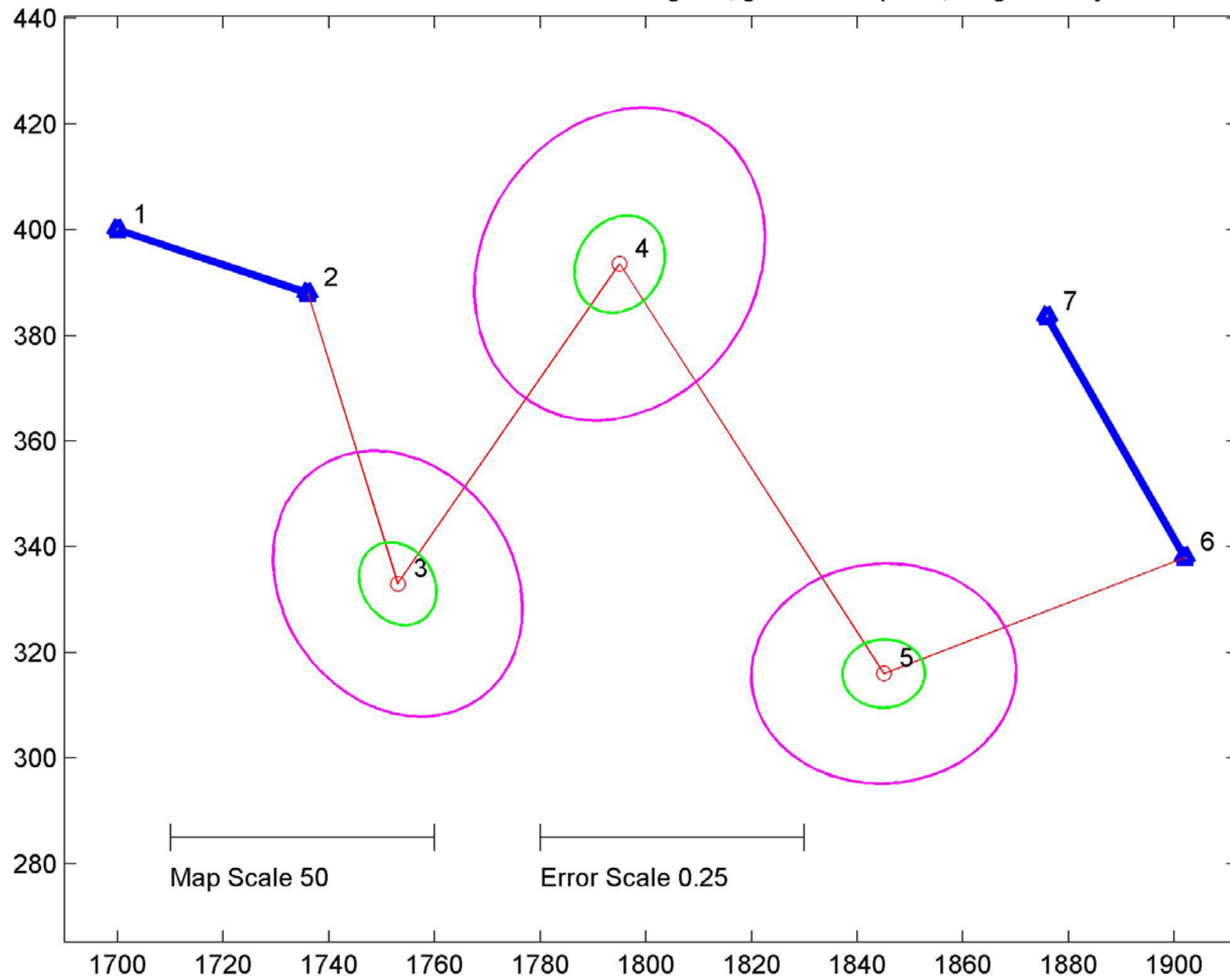
HW4 / HW6 Traverse Plot with 99% conf. regions, green=accept Ho, magenta=reject
