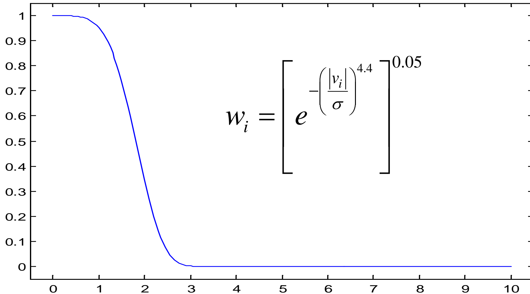
IRLS weight function #1
