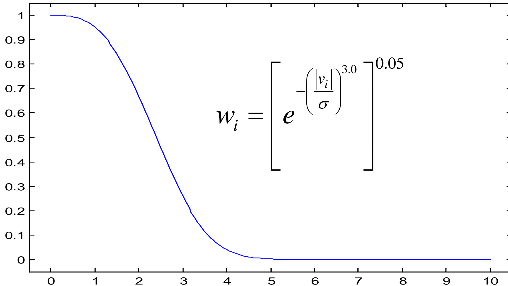
IRLS weight function #2
