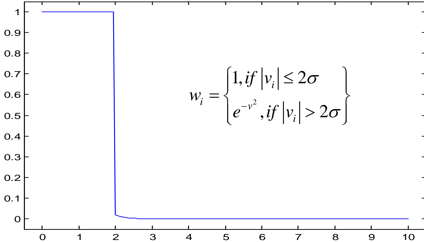
IRLS weight function #3
