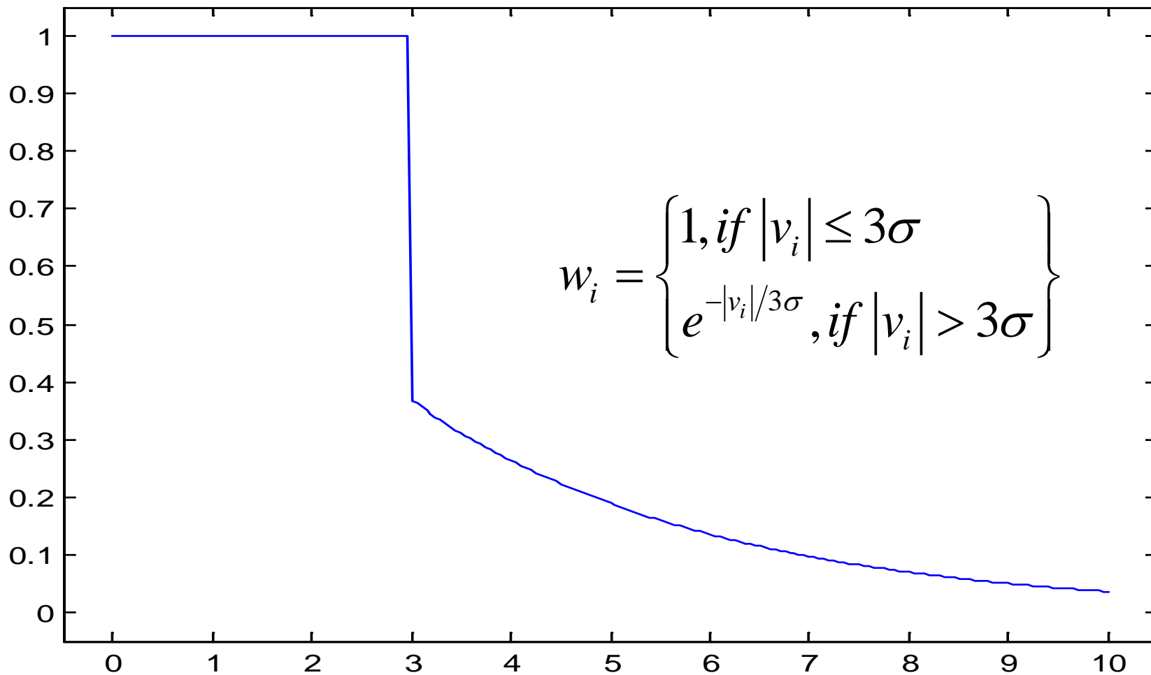
IRLS weight function #4
