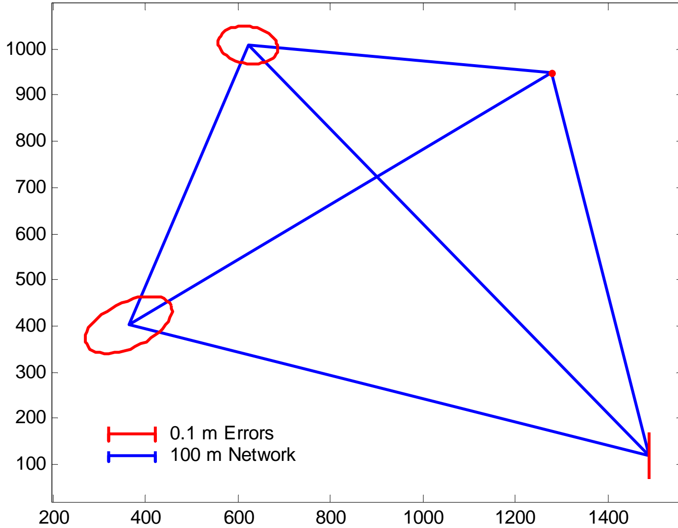
Plot of Braced Quad: Network and Errors
