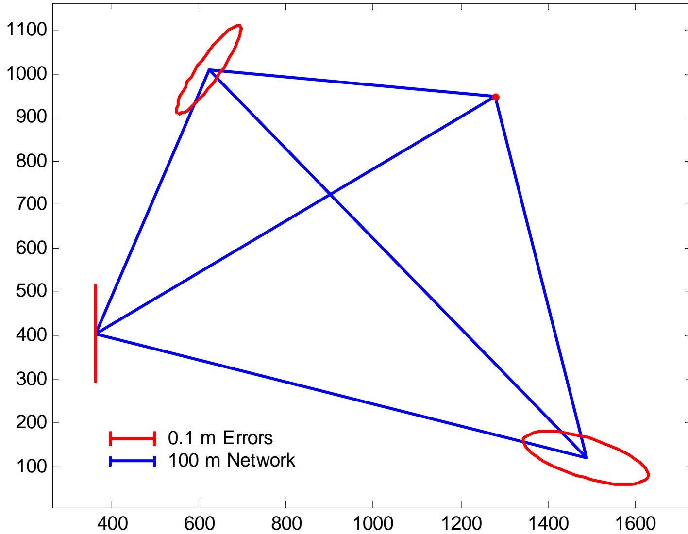
Plot of Braced Quad: Network and Errors
