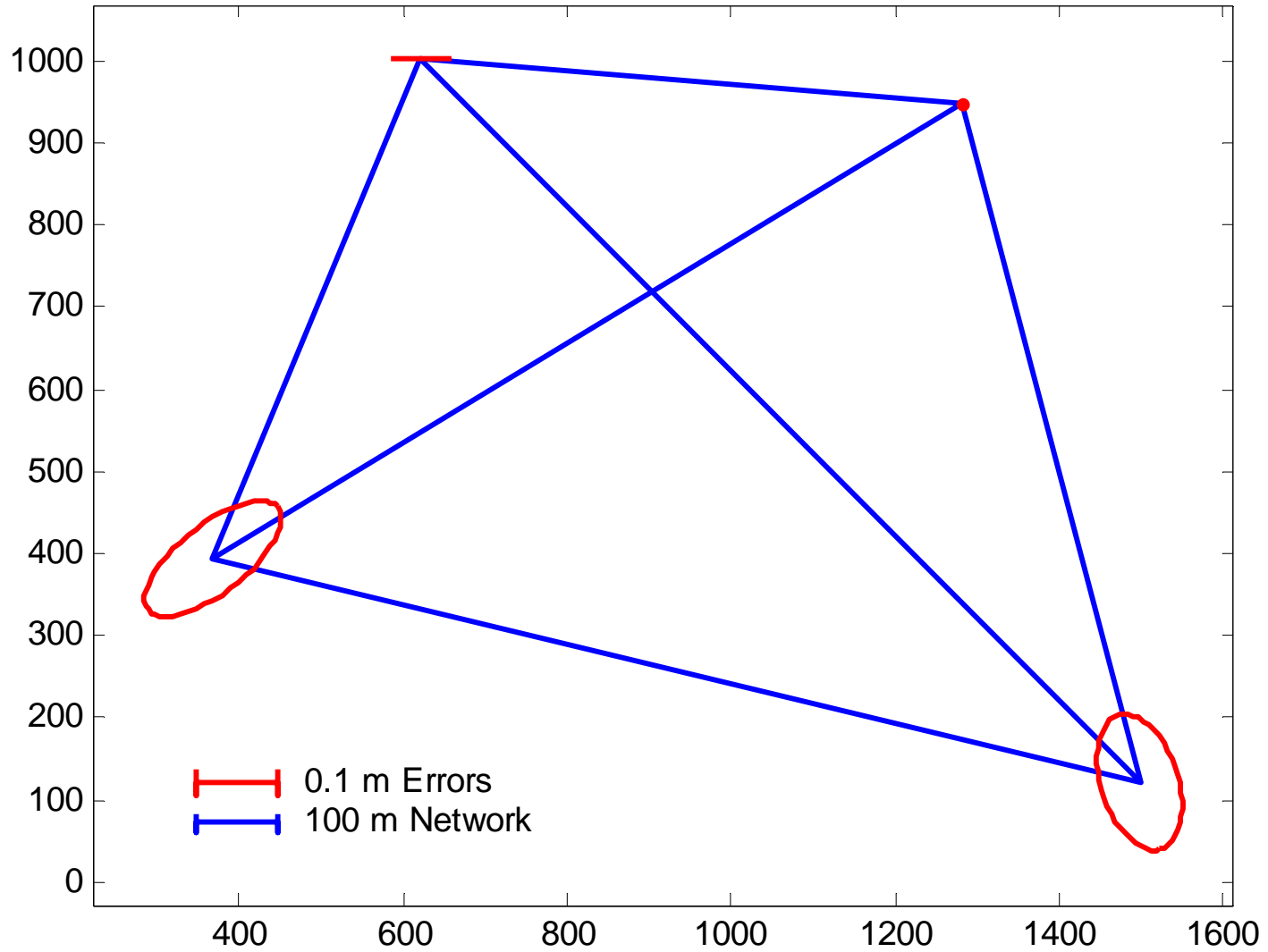
Plot of Braced Quad: Network and Errors
