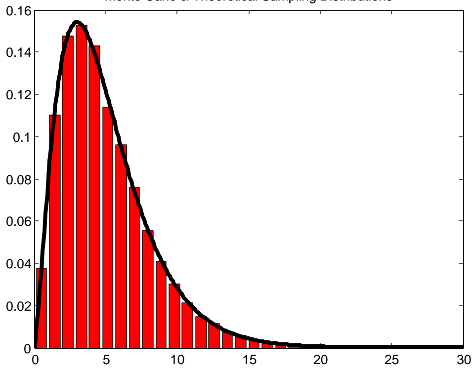
Monte Carlo & Theoretical Sampling Distributions
